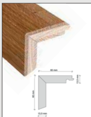
Stair nosing with connection on one side
