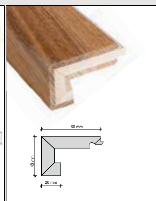
Stair nosing, angled
